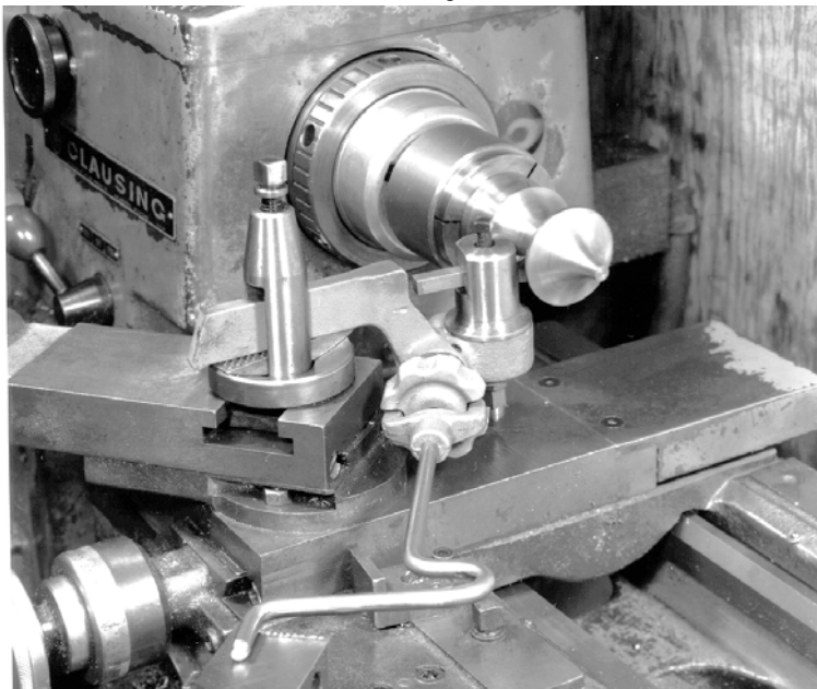
The No. A1-248-07 SHAPLANE Radius Tool turning a concave radius.
